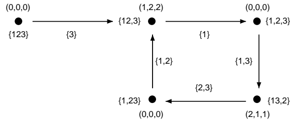
Figure 3. The largest cautious consistent set might be empty.
