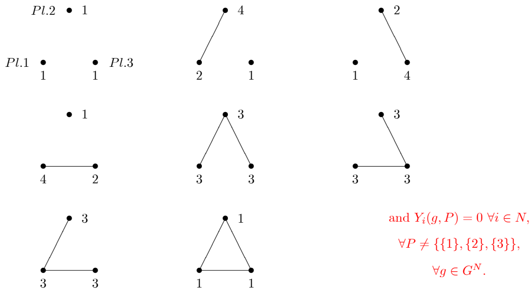
Figure 4: Non-existence of contractually stable networks
