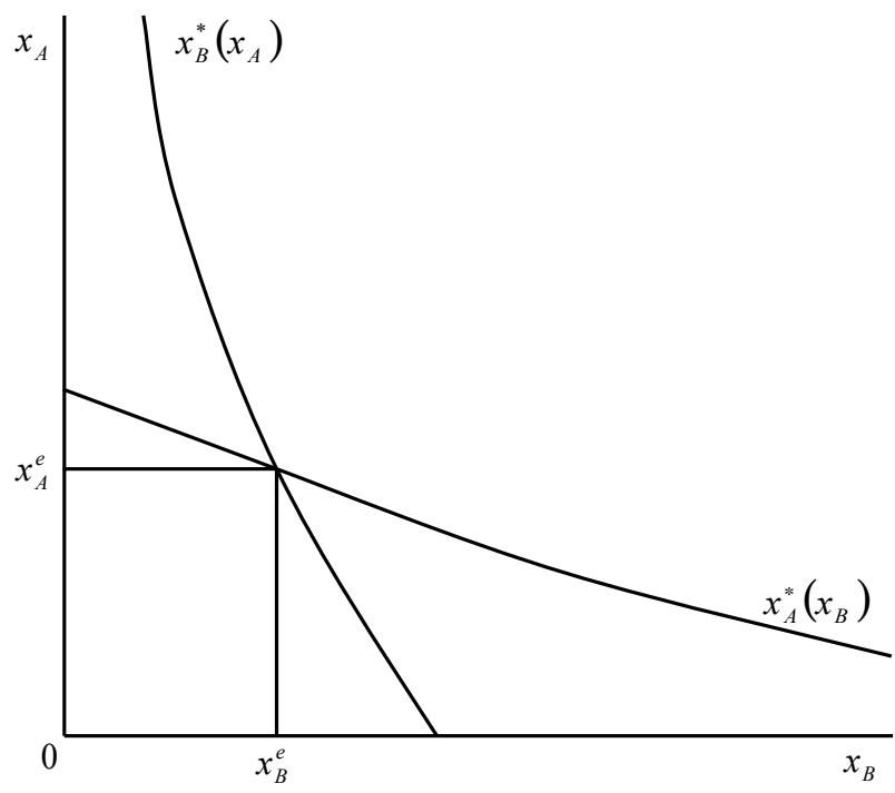
Figure 2. The uniqueness of the equilibrium
