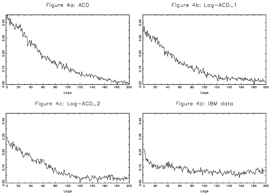
FIGURE 4 Autocorrelation Functions of 3 Simulated Data Sets Corresponding to ACD, Log-ACD 1 and Log-ACD 2 Specifications, and for the IBM Data.
