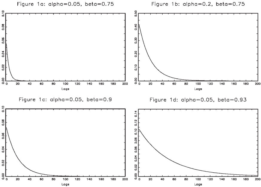
FIGURE 1 Autocorrelation Functions of the ACD Model
